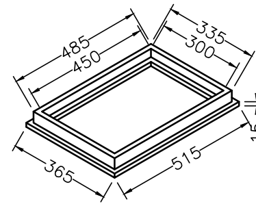
ISOMETRIC
